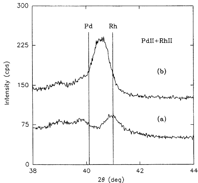
Figure 3. XRD patterns obtained from PdII + RhII after aging (a), followed by mild reduction (b).
